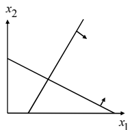
unbounded polyhedron
