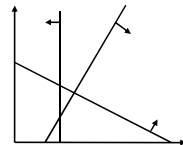
empty polyhedron
